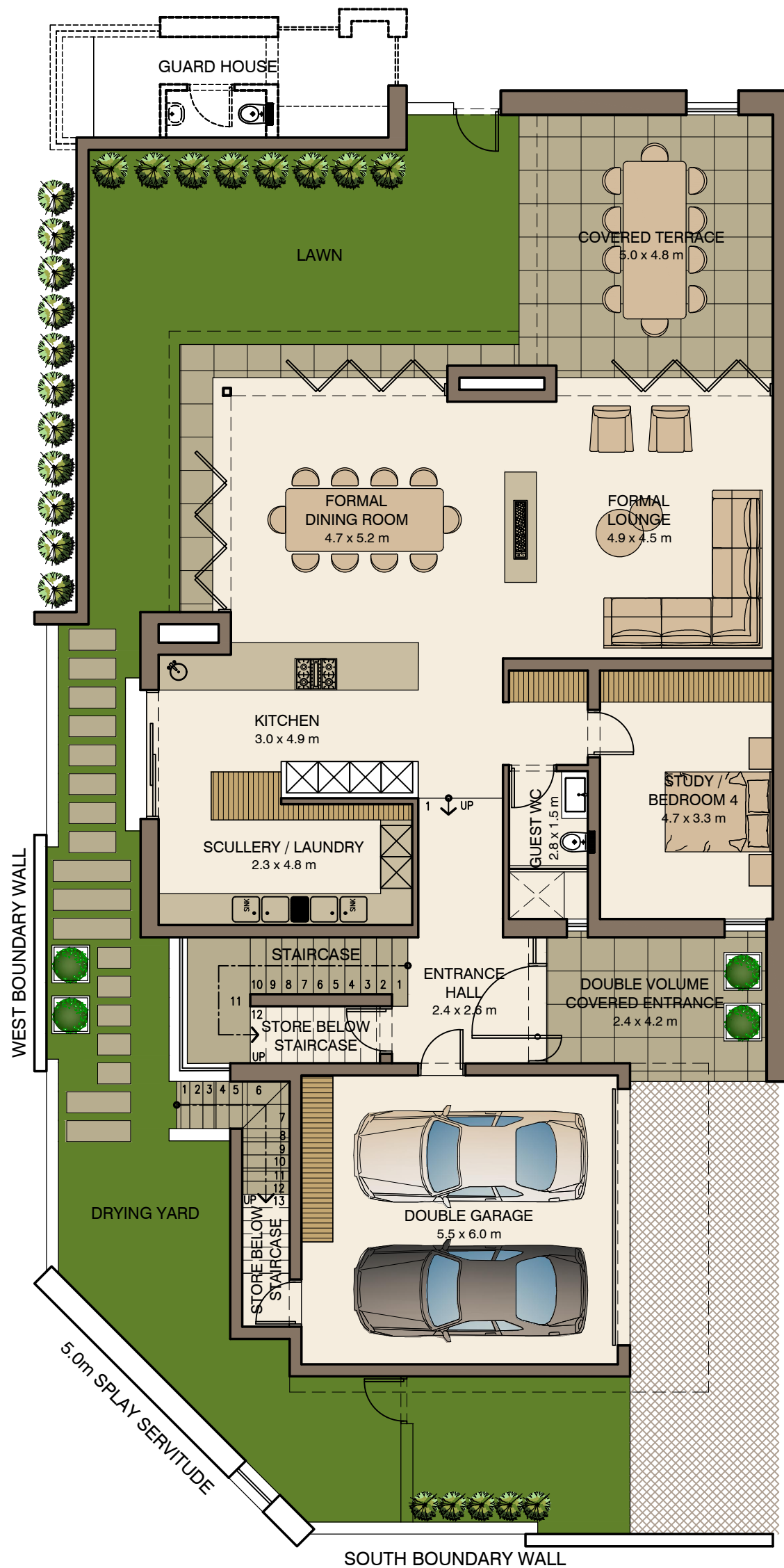
GROUND FLOOR PLAN NOT TO SCALE
