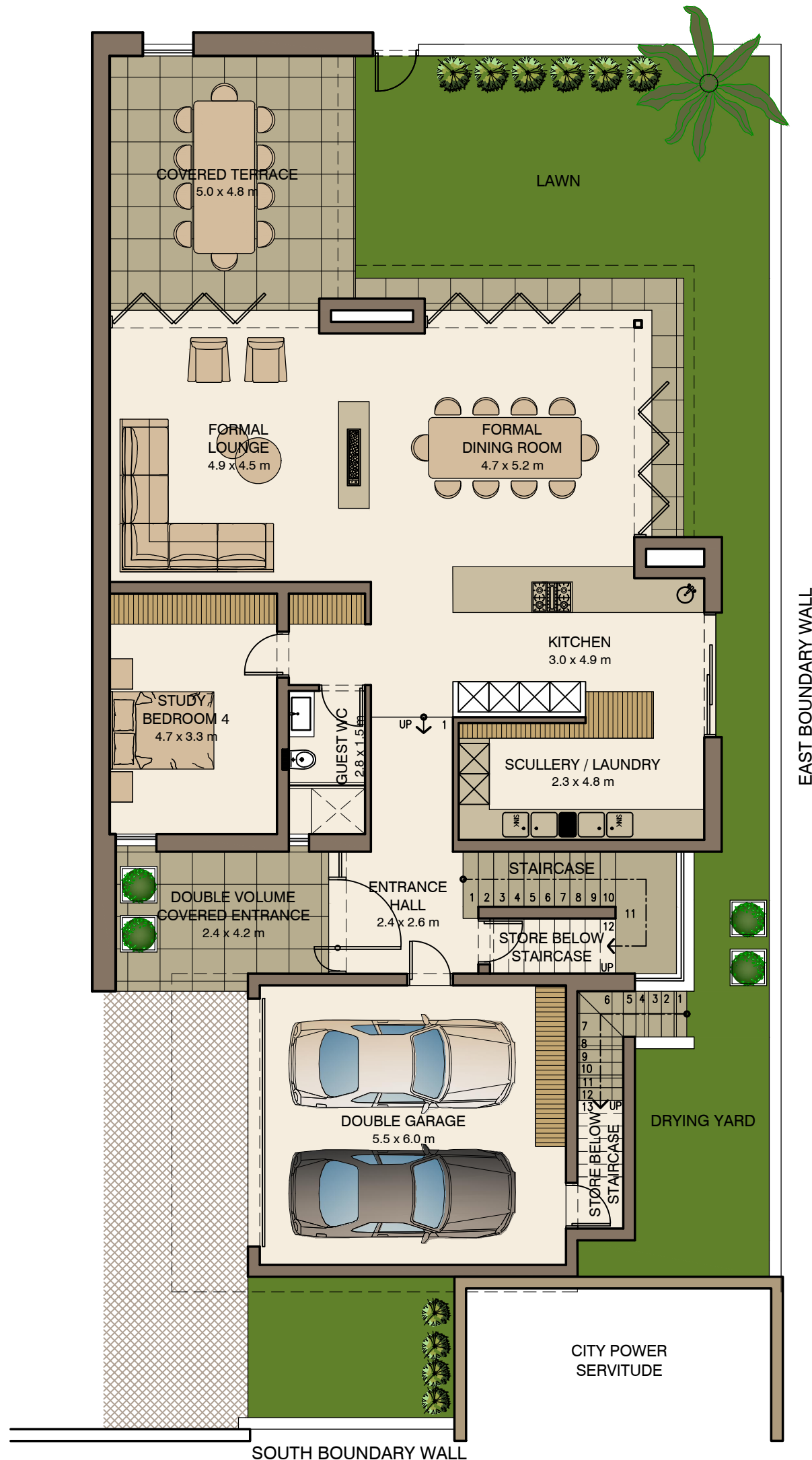
GROUND FLOOR PLAN NOT TO SCALE
